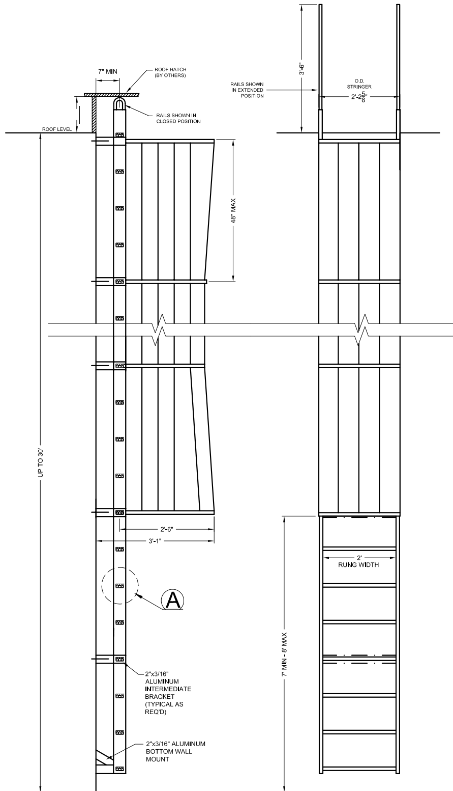
SECTION 3/8" = 1'-0"
