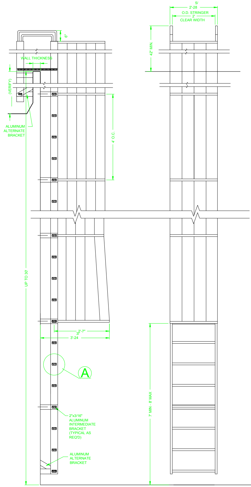
SECTION 3/8" = 1'-0"
