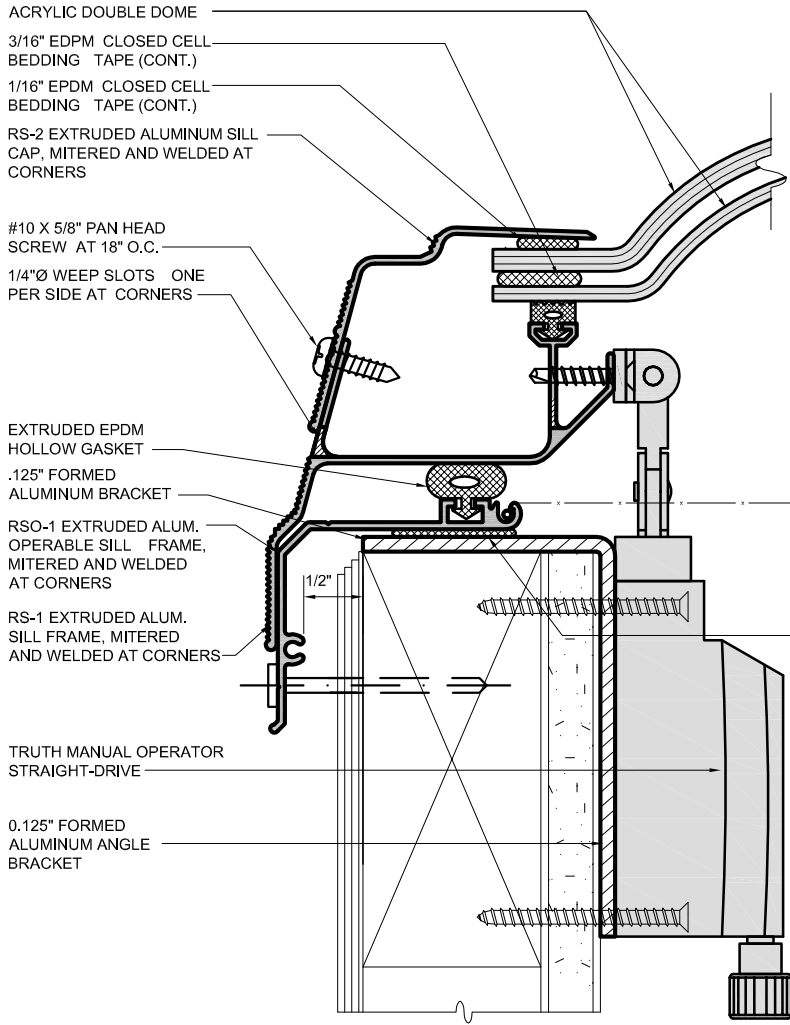
1 1 SILL @ OPERABLE SECTION SCALE 0 1"
