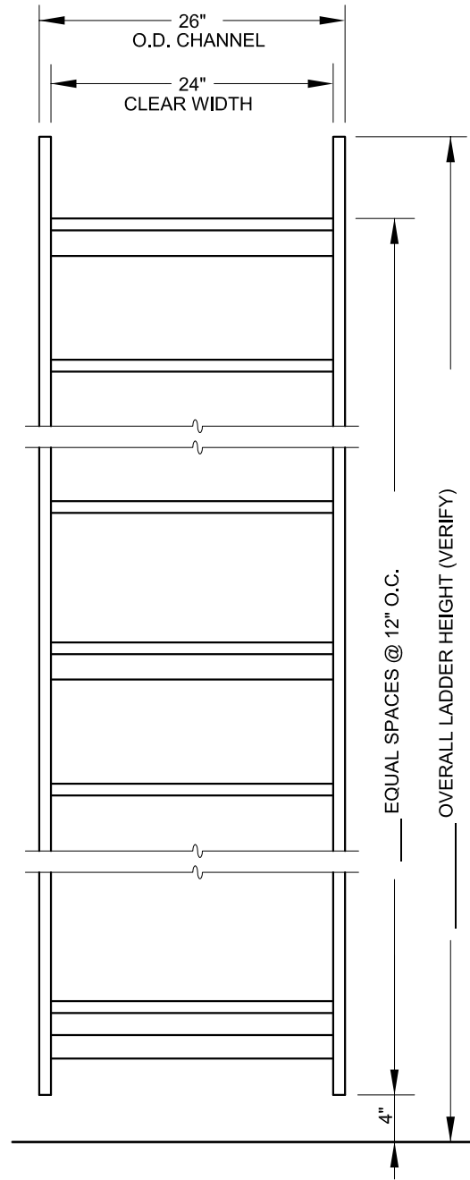
FRONT ELEVATION 3/4" = 1'-0"
