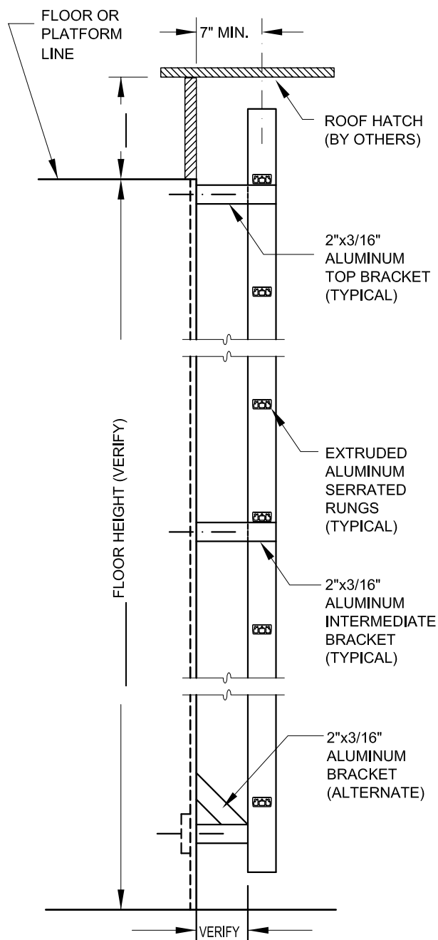
SECTION 3/4" = 1'-0"
