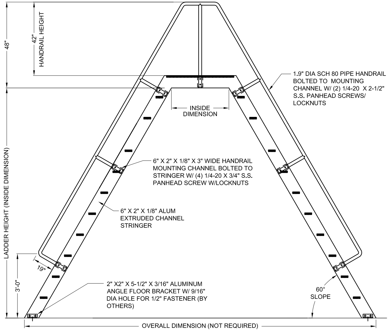
SIDE ELEVATION 3/8" = 1'-0"
