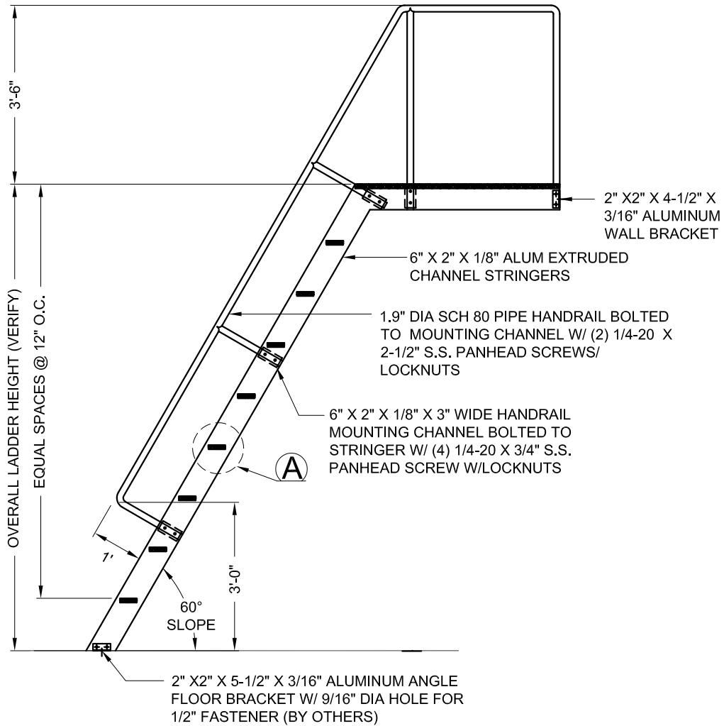
SIDE ELEVATION 3/8" = 1'-0"
