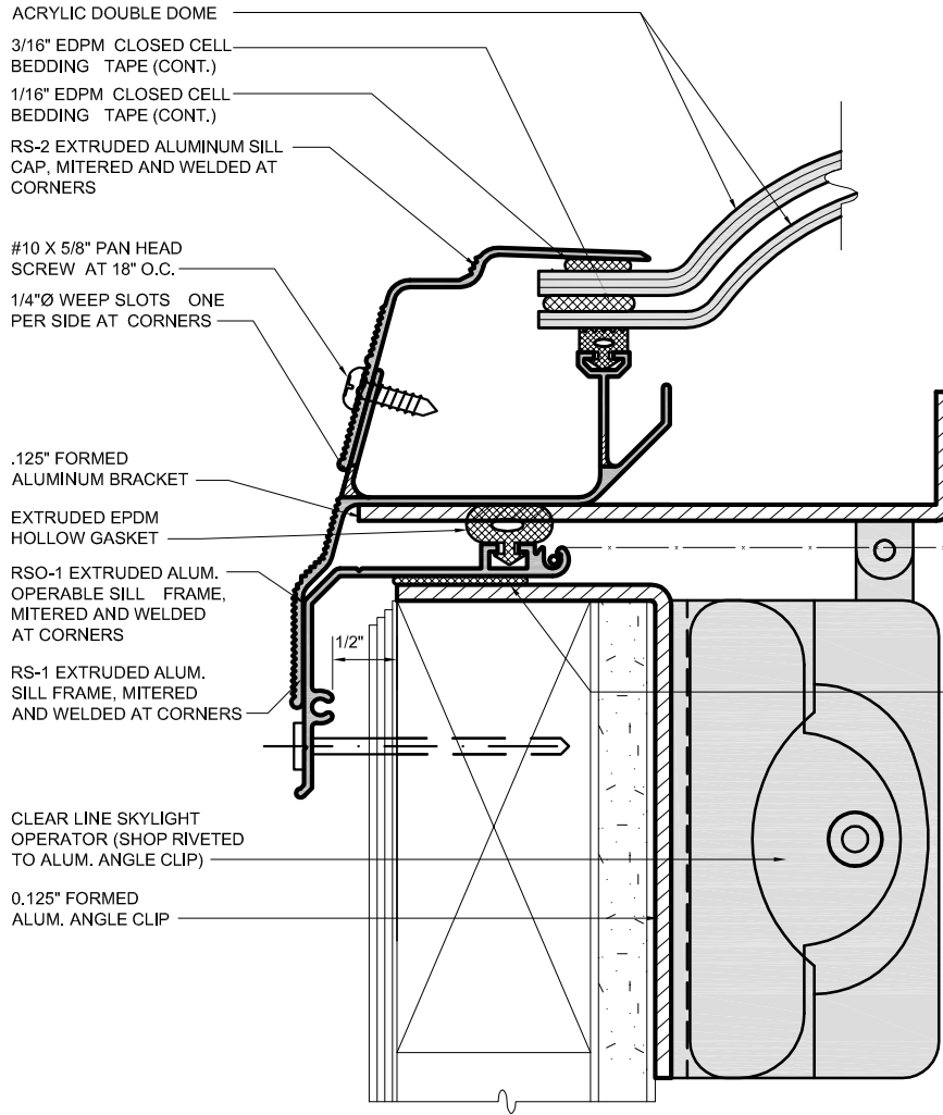
1 1 SILL @ OPERABLE SECTION SCALE 0 1"
