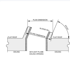
Flat roof 1:12 min – 2:12 max pitch
