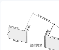
Plumb ceiling opening Curb square to the roof, plumb opening below
